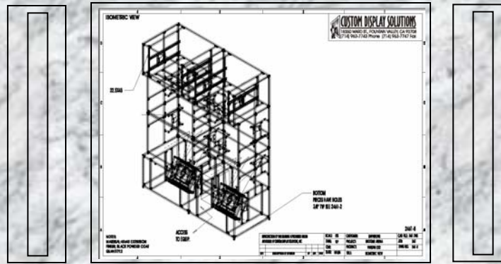
DESIGN – ISOMETRIC
