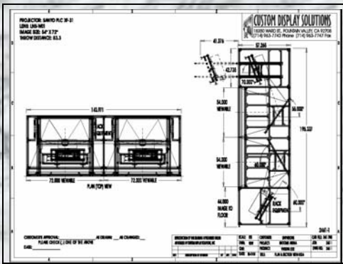
DESIGN – PLAN & SECTION
